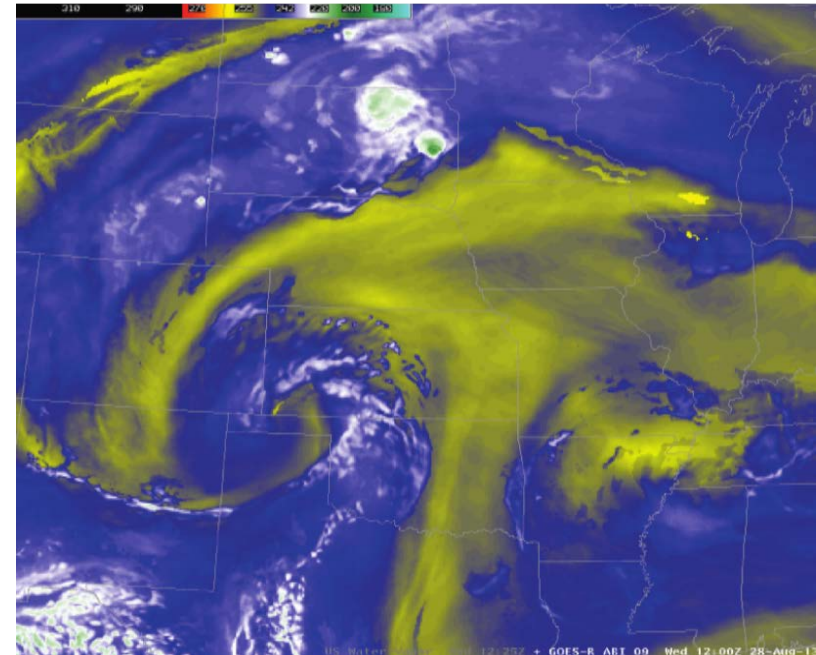
Synthetic ABI Band 09 Imagery
